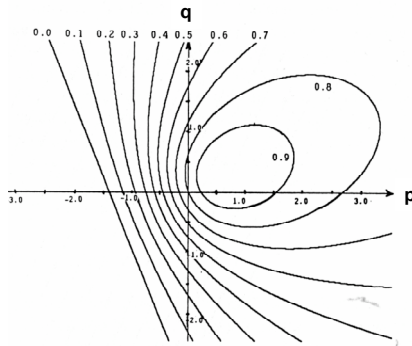
Reflectance map for Lambertian surface illuminated from p_i = 0.7 and q_i = 0.3
