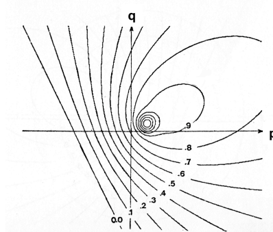
Reflectance map for matte surface with specular component
