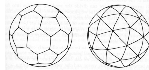
truncated icosahedron (left) provides 12 pentagonal and 20 hexagonal faces, pentakis dodecahedron (right) provides 60 triangular faces
