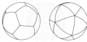
dodecahedron (left) and icosahedron (right) provide tessellations with 12 and 20 cells, respectively
