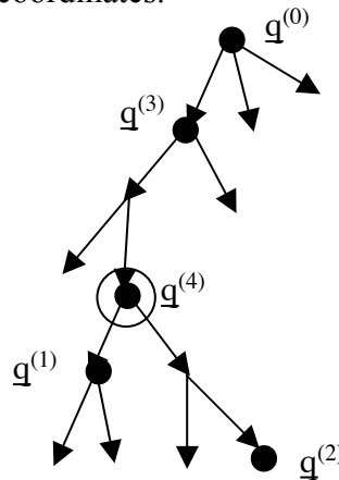
Figure 7: Updating probabilities in a BCH for evidence in absolute coordinates
