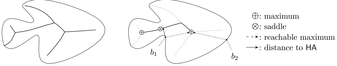
Figure 1: left: medial axis, right: our new homotopical axis (illustrated in 2D for simplicity)
