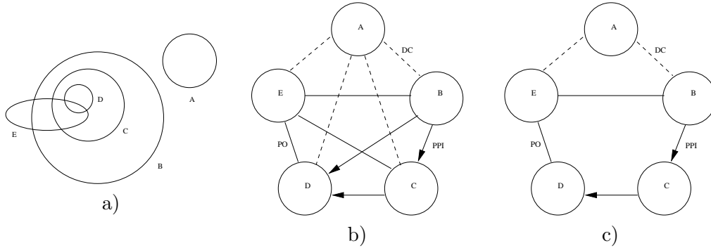
Figure 3: a) Scene, b) corresponding RCC5 net, c) edge-reduced RCC5 net
