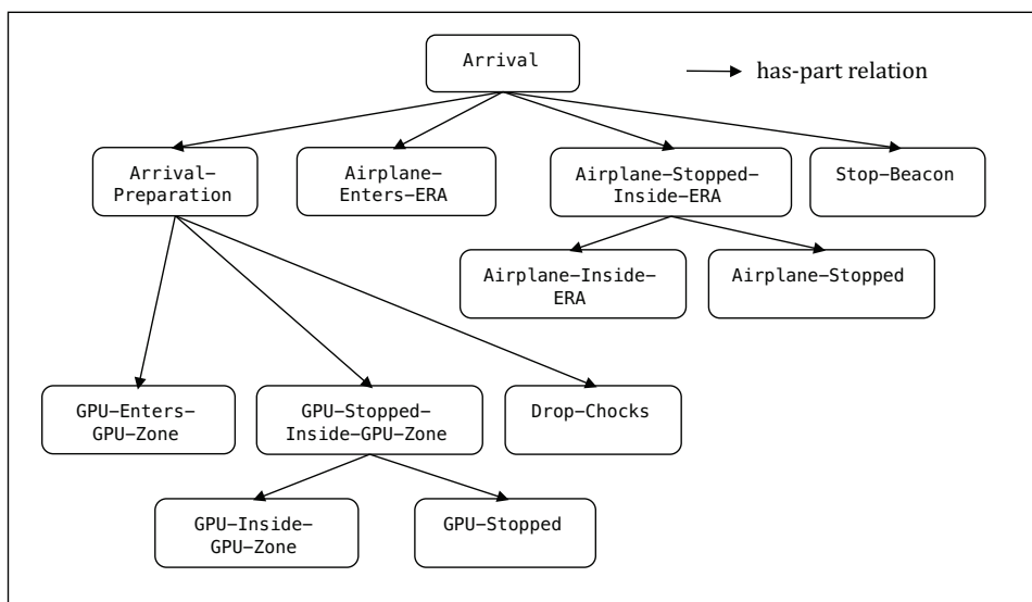
Fig. 4: Hypotheses graph for the submodel Arrival
