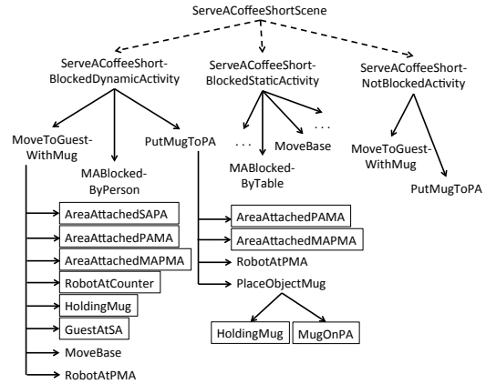
Figure 4: A multi-level compositional structure. Solid edges represent conjunctive properties, dotted edges disjunctive properties.
