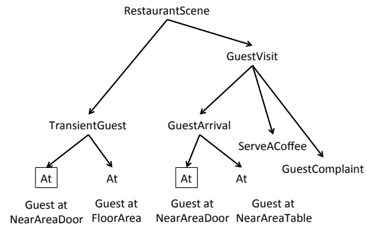
Figure 7: Model of guest visit.
