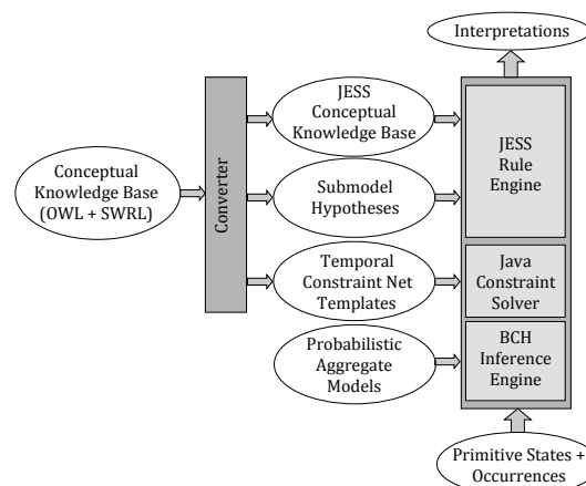
Figure 2: Components of SCENIOR scene interpretation system.
