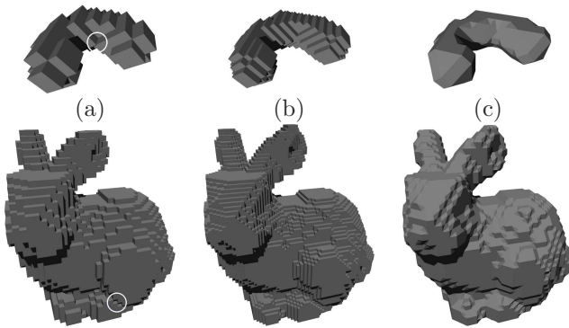
Figure 6. Different reconstruction algorithms: (a) digital reconstruction (Note that the surface is not a manifold inside the circle) (b) majority interpolation, (c) modified marching cubes.
