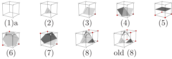
Figure 5. Cases 1 to 8 for the MMC algorithm and case 8 for the original Marching Cubes algorithm.
