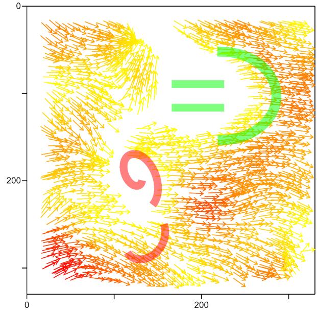
(a) Derived sea surface currents
