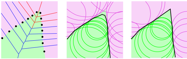
Figure 11. The inner poles of the samples near a sharp corner do not pass the ‘skininess’ test. But just discarding the inner poles collapses the power crust at the corner. Discarding both poles of the badly-shaped Voronoi cells allows the power crust faces formed in nearby well-sampled regions to extend into the region of uncertainty and meet at a sharp corner.
