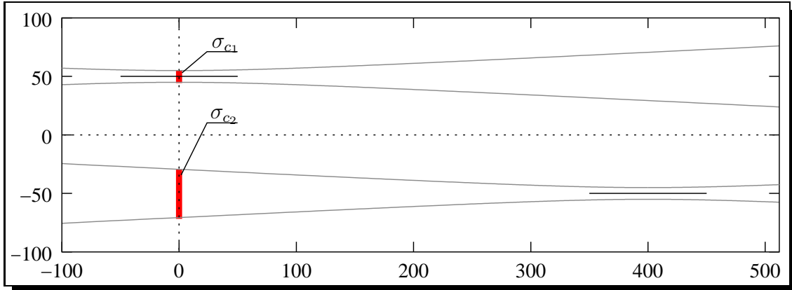
Figure 4.20: The uncertainty in the distance from the origin c depends on the location of the line segment line segment .
