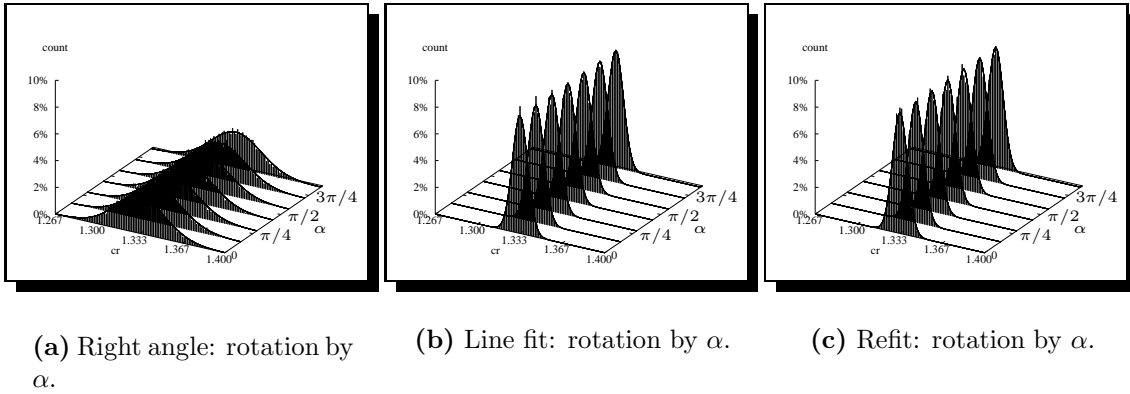
Figure 4.14: Measured and predicted distribution of the crossratio for three different algorithms and varying angle of rotation \alpha .
