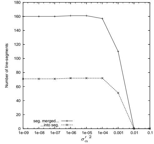
Figure 6.16: Number of line segments line segments that got merged, and number of line segments line segments they got merged into, for different values of \sigma'_\alpha{}^2 .
