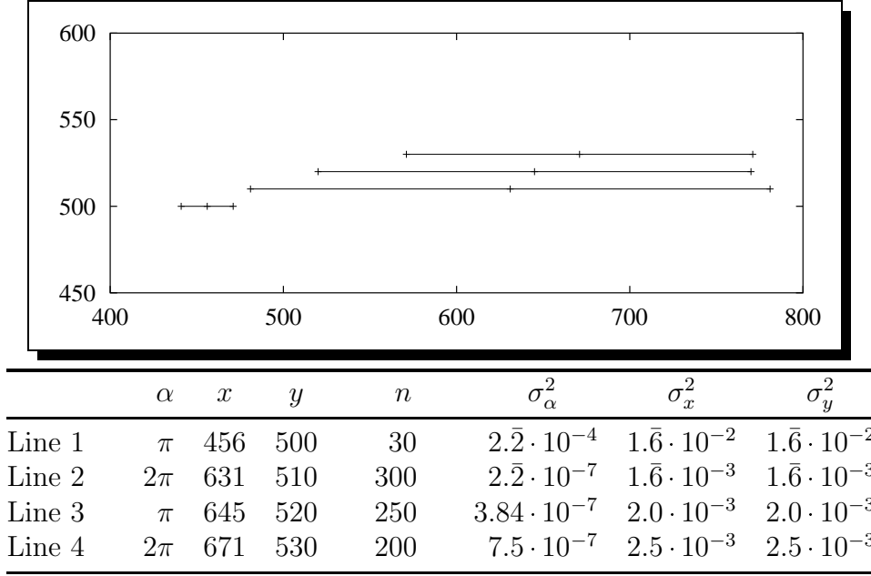
Figure 4.13: Dataset Data set used for Monte-Carlo simulations (cross-ratio).
