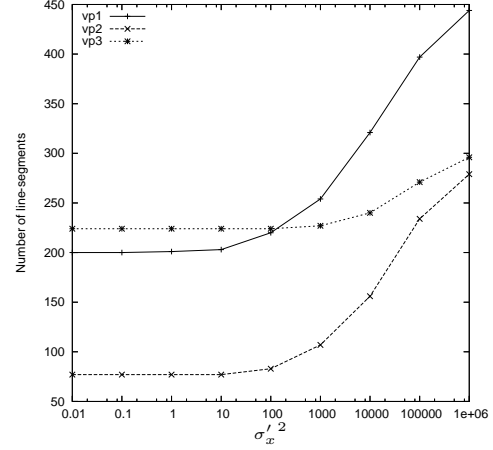
Figure 6.14: Number of line segments line-segments classified as belonging to each of the three vanishing points vanishing points for different values of \sigma'_x{}^2 .
