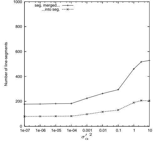
Figure 6.18: Number of line segments line segments that got merged, and number of line segments line segments they got merged into, for different values of \sigma'_\alpha{}^2 and a fixed maximum distance between segments of 500 pxl.
