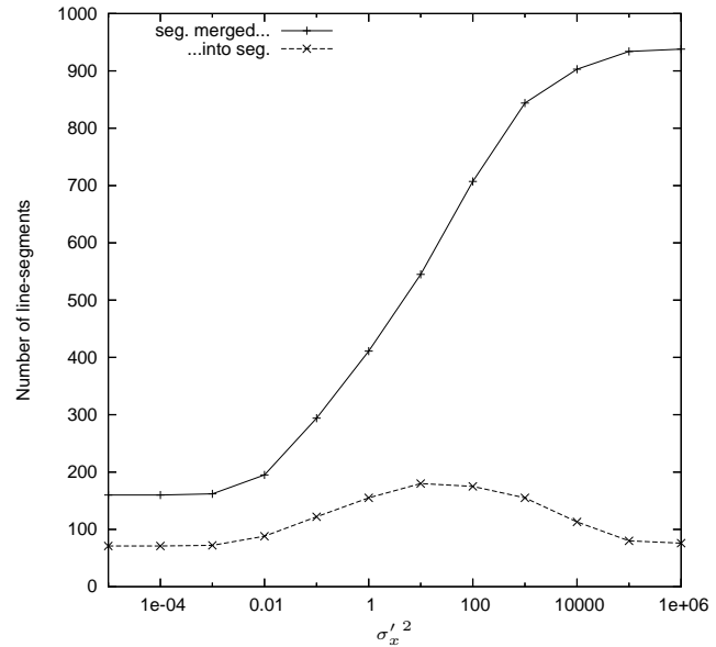
Figure 6.17: Number of line segments line segments that got merged, and number of line segments line segments they got merged into, for different values of \sigma'_x{}^2 .
