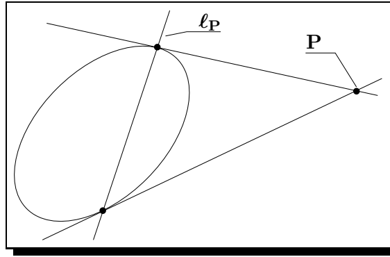
Figure 2.11: Pole and polar of a conic.
