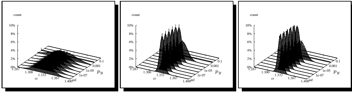
(a) Right angle: projective distortion p_y .
