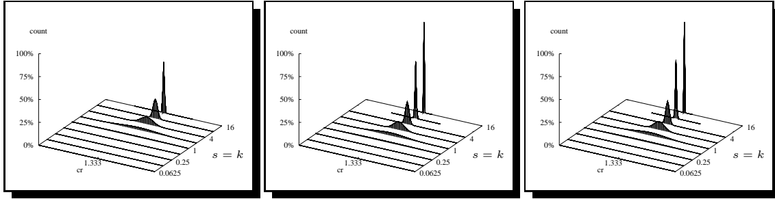
(a) Right angle: resolution s = k .
