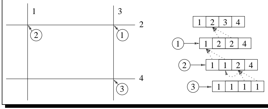
Figure 6.4: Labelling line segments line-segments within a mesh can require recursive look-up of labels.
