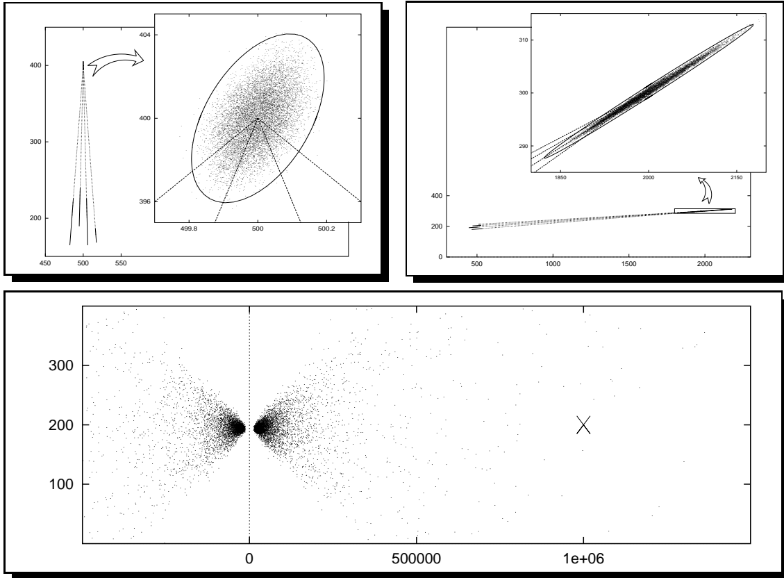
Figure 4.9: Monte Carlo simulation of the calculation of line-intersections for three typical constellations. The two top figures demonstrate how well the theoretically derived covariance matrix covariance matrix (the ellipses, enclosing 99 % of all points) and the Monte-Carlo simulation agree for intersections close to the image. The bottom figure shows that for far away intersections (×) the covariance-region becomes hyperbolic in Euclidean coordinates, which is poorly modelled by Gaussian noise.
