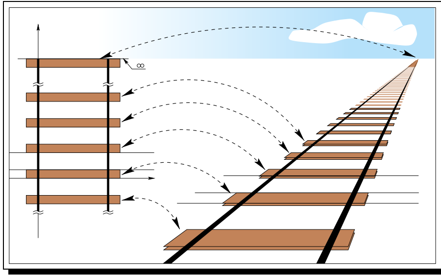
Figure 5.10: Finding additional line segments line-segments by backprojection.
