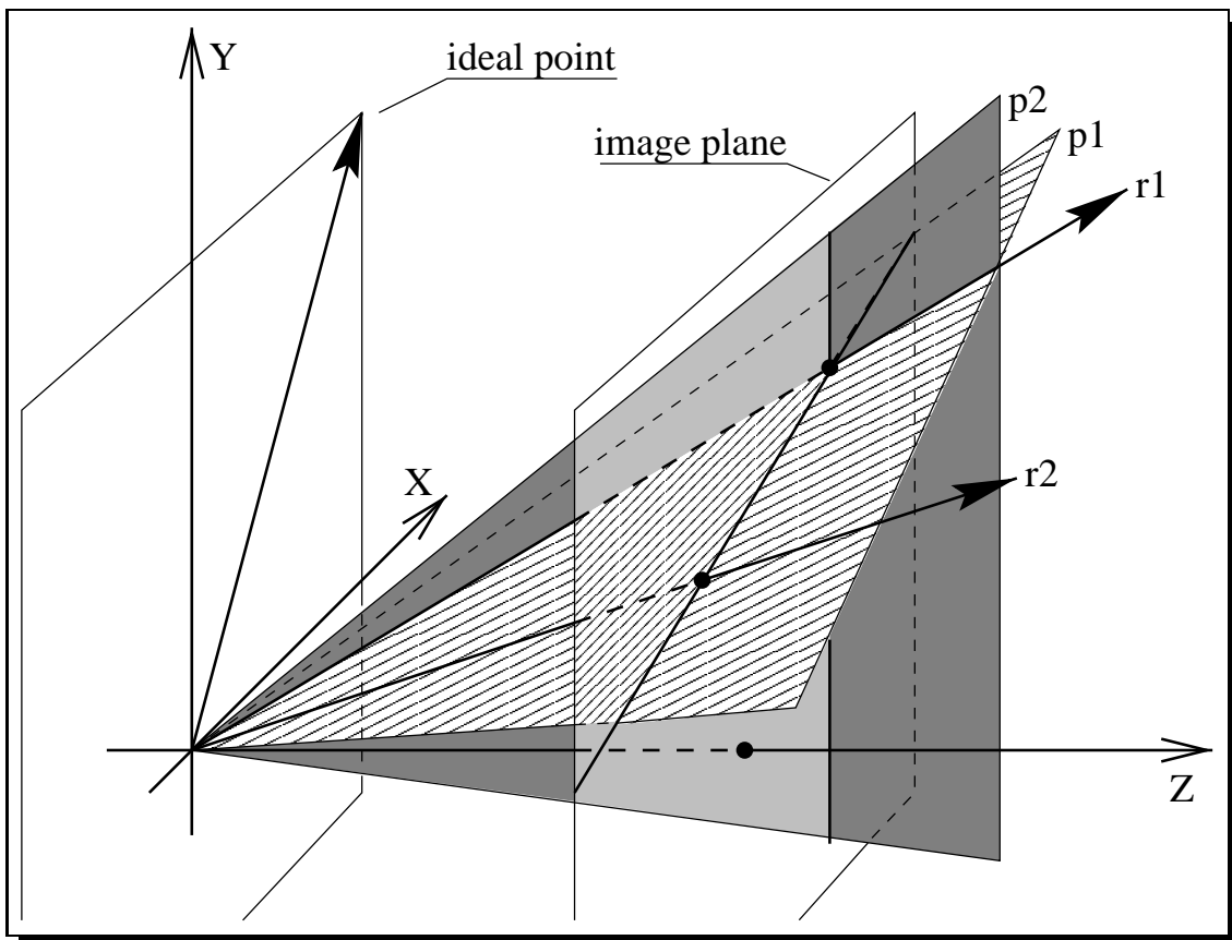
Figure 2.18: Ray-space model. Each ray corresponds to a point in the image plane. Two rays span a plane, two planes define a ray. Ideal points correspond to a ray parallel to the image plane image plane .
