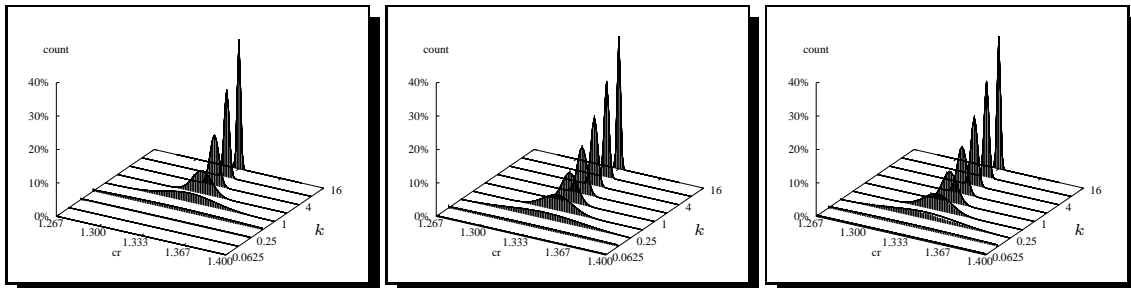
(b) Line fit: accuracy k .
