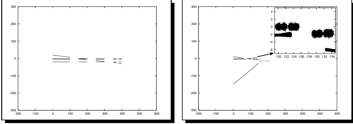
Figure 6.8: Experimental setup containing collinear line segments line segments (left) and maximally distorted set (right). The inset detail shows how widely the smallest line segments line segments vary in both position and orientation; line segments line segments that small would not be used in practical applications but rather help to analyse border-line conditions.
