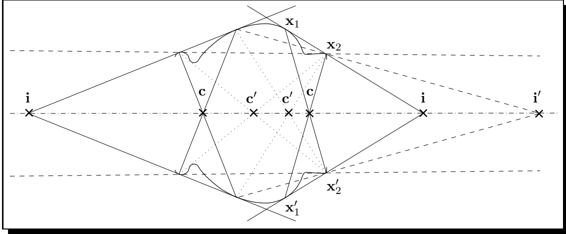
Figure 7.5: Features used: bitangent intersections are marked i , crosspoints are marked c . The points marked i' and c' are interpair inter-pair -features.
