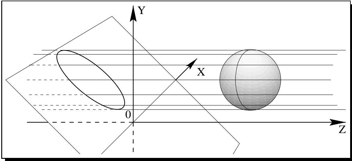
Figure 2.6: The affine camera. Movement of the image plane image plane around the origin (plus scaling) is equivalent to an affine transformation of the image plane image plane .
