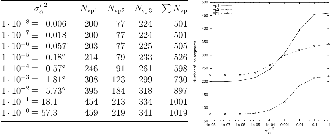
Figure 6.13: Number of line segments line segments classified as belonging to each of the three vanishing points vanishing points for different values of \sigma'_\alpha{}^2 .
