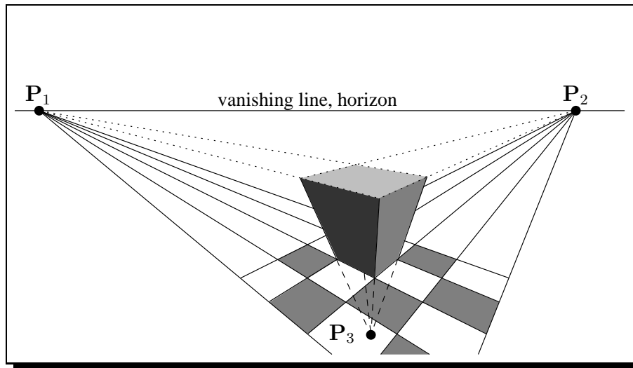
Figure 2.9: Vanishing points Vanishing points and vanishing line vanishing line .
